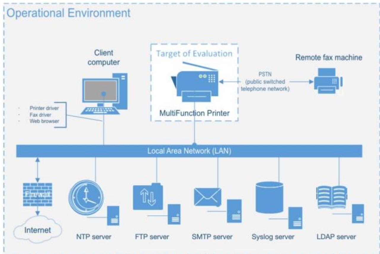
Figure 1: TOE Architecture
